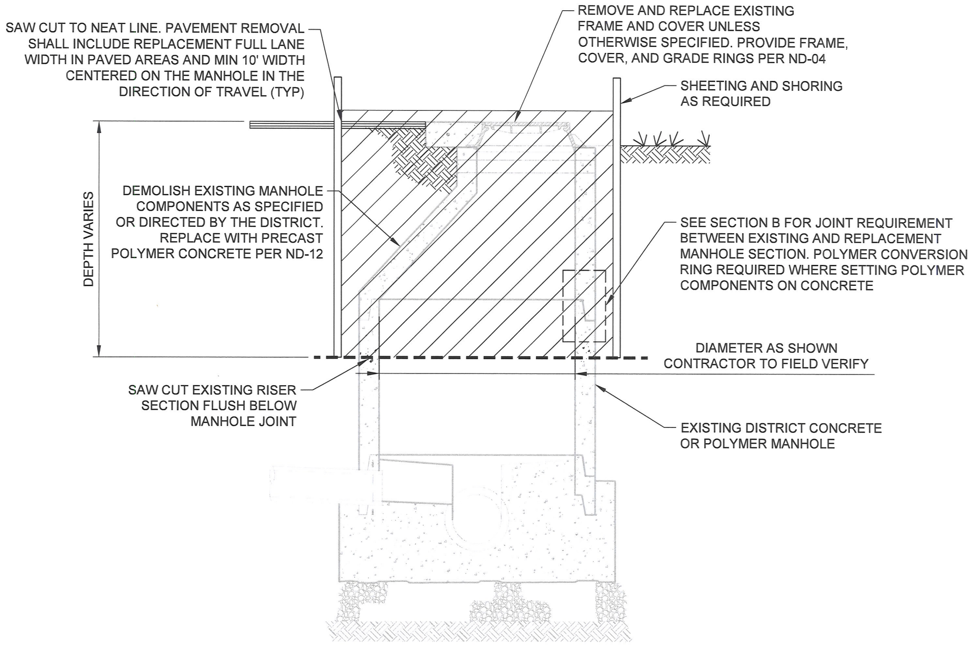
SECTION A
